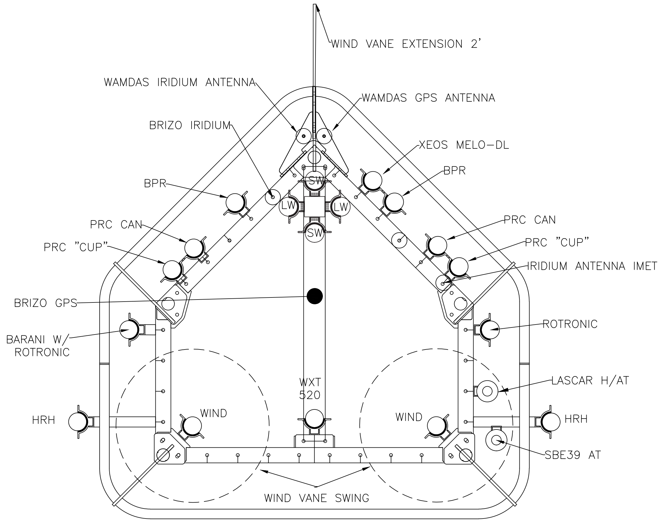
NTAS 17 TOWER TOP V4 4/24/18 BP
