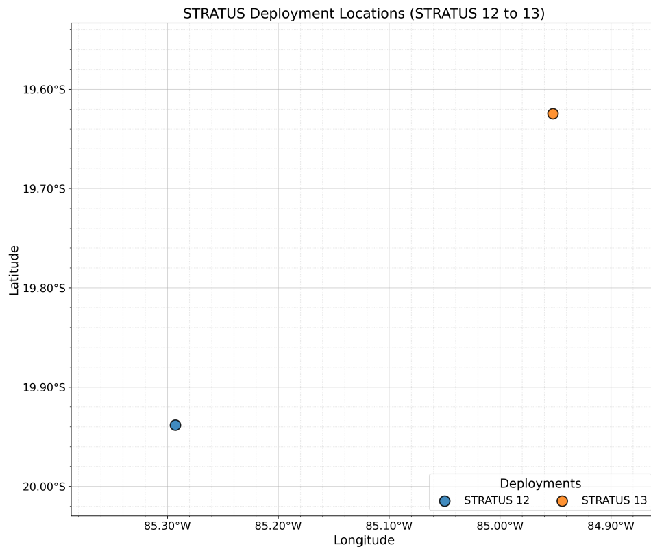
Figure 8: Deployment locations for Stratus moorings from Stratus 12 to Stratus 13. The map shows the anchor positions determined during deployment surveys.
