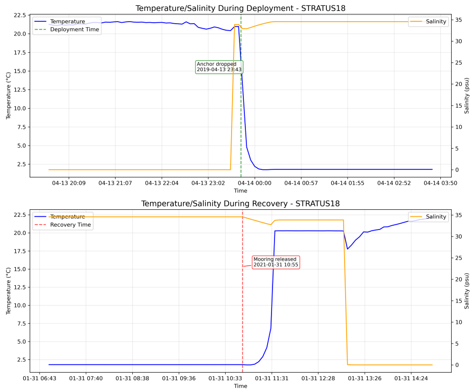
Figure 3: Detailed view of temperature changes during deployment and recovery phases for stratus 18, showing instrument SBE37 10600.
