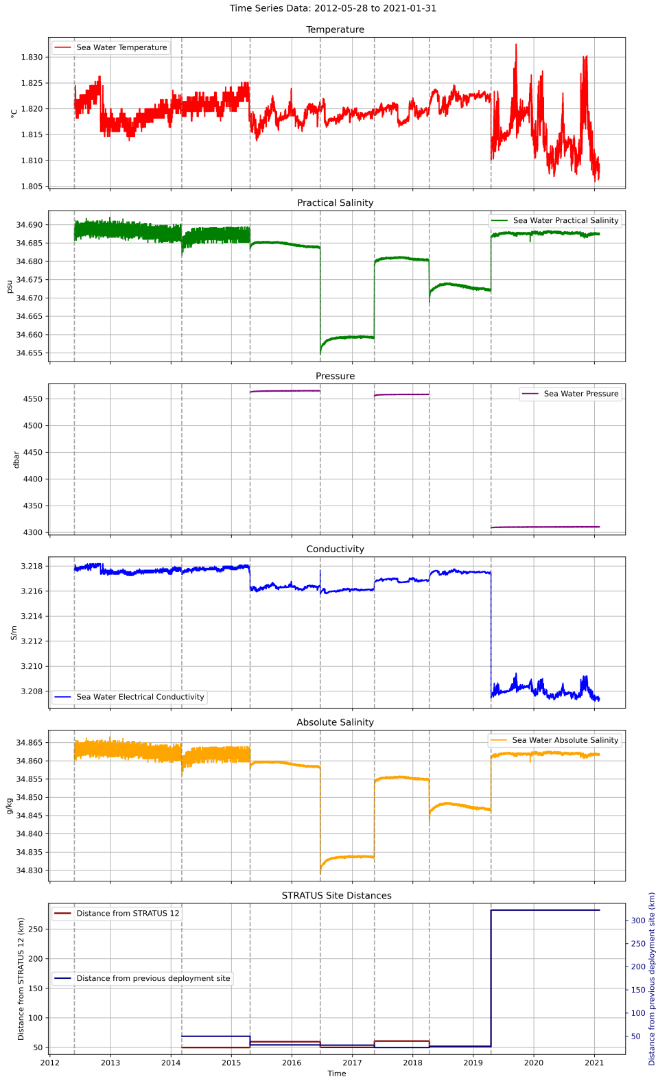
Figure 10: Merged dataset of stratus 12 to stratus 18 showing the transition at the merge point. This dataset combines data from the selected instrument (SBE37 12257) from stratus 17 and SBE37 10600 from stratus 18. This dataset incorporates all previous merges in the time series.
