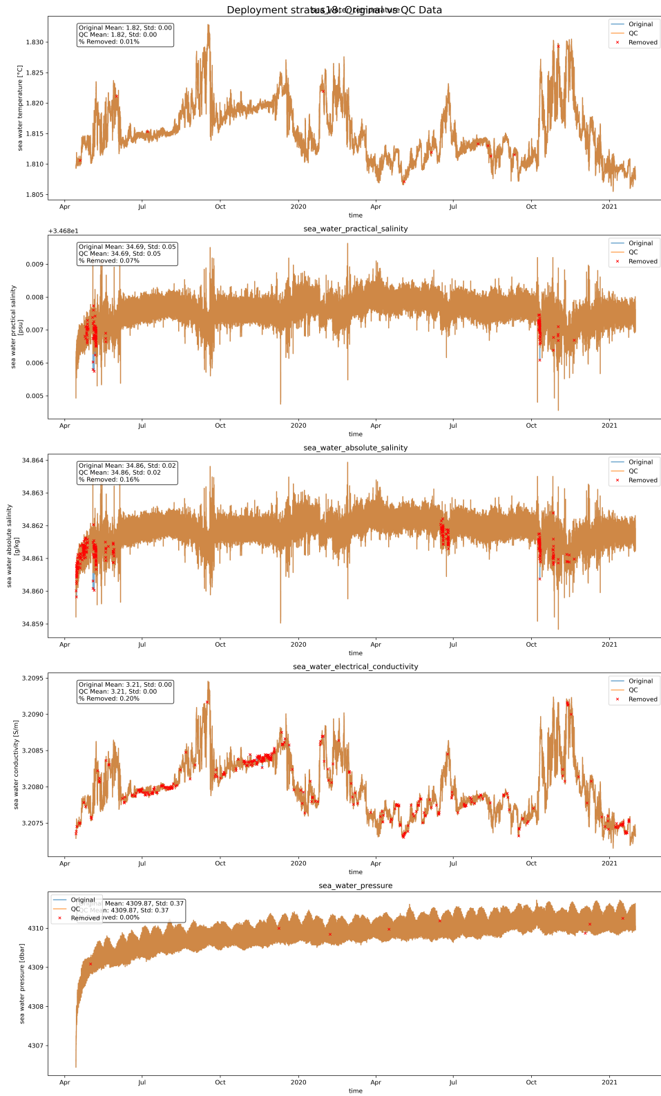
Figure 6: Original and clean plots of temperature, salinity, absolute salinity, conductivity, and pressure for instrument SBE37 10600 of stratus 18.
