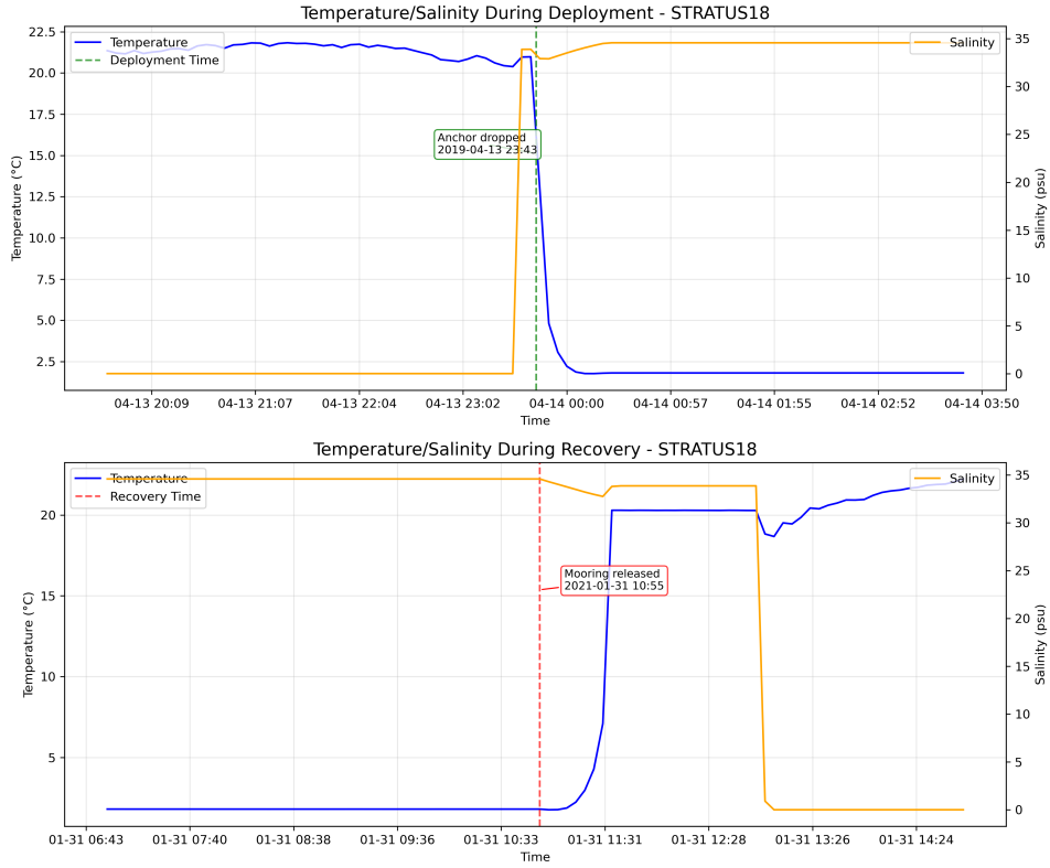
Figure 4: Detailed view of temperature changes during deployment and recovery phases for instrument SBE37 10601 of stratus 18.
