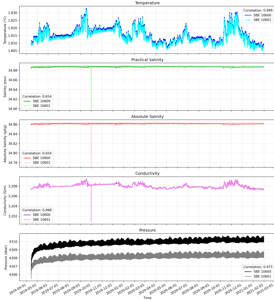
Comparison within STRATUS18 Data Location: (22.4626°S, 85.6598°W) | Depth: 4229m
