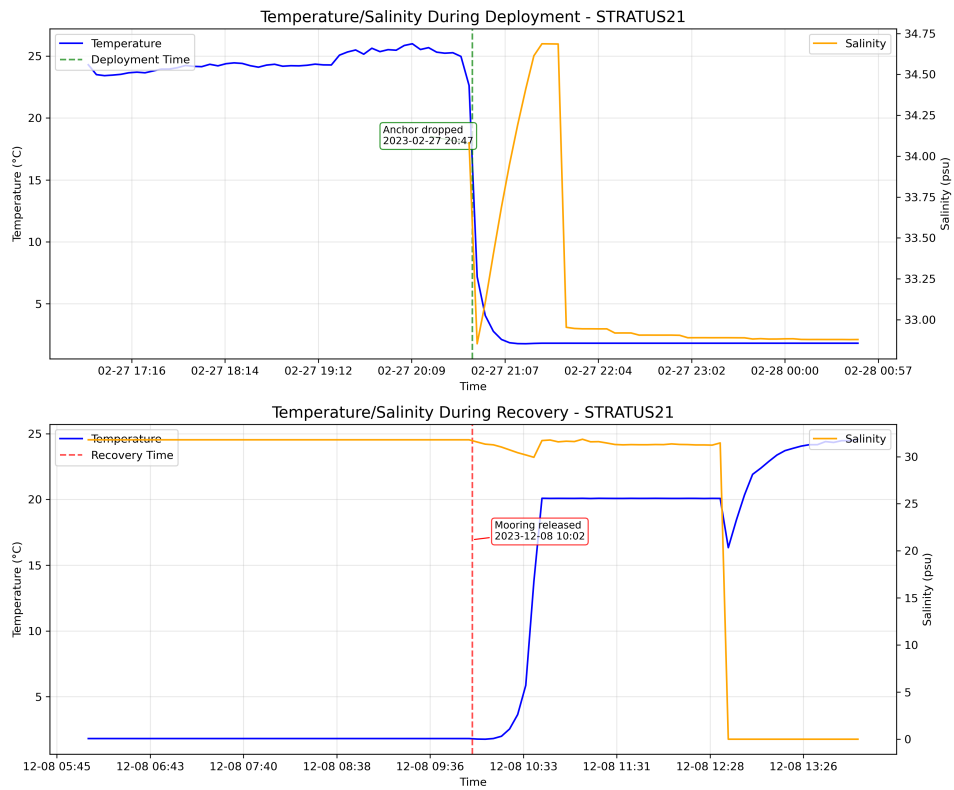
Figure 3: Detailed view of temperature changes during deployment and recovery phases for stratus 21, showing instrument SBE37 11379.
