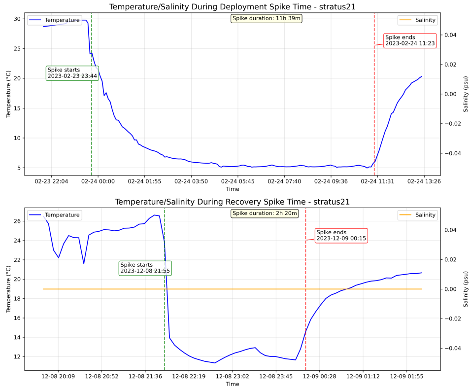
Figure 1: Deployment and recovery spike times for instrument SBE37 11379 of stratus 21 showing temperature changes during deployment and recovery operations. The vertical dashed lines indicate the recorded spike times (2023/02/24 11:23:00 for deployment and 2023/12/08 21:55:00 for recovery).
