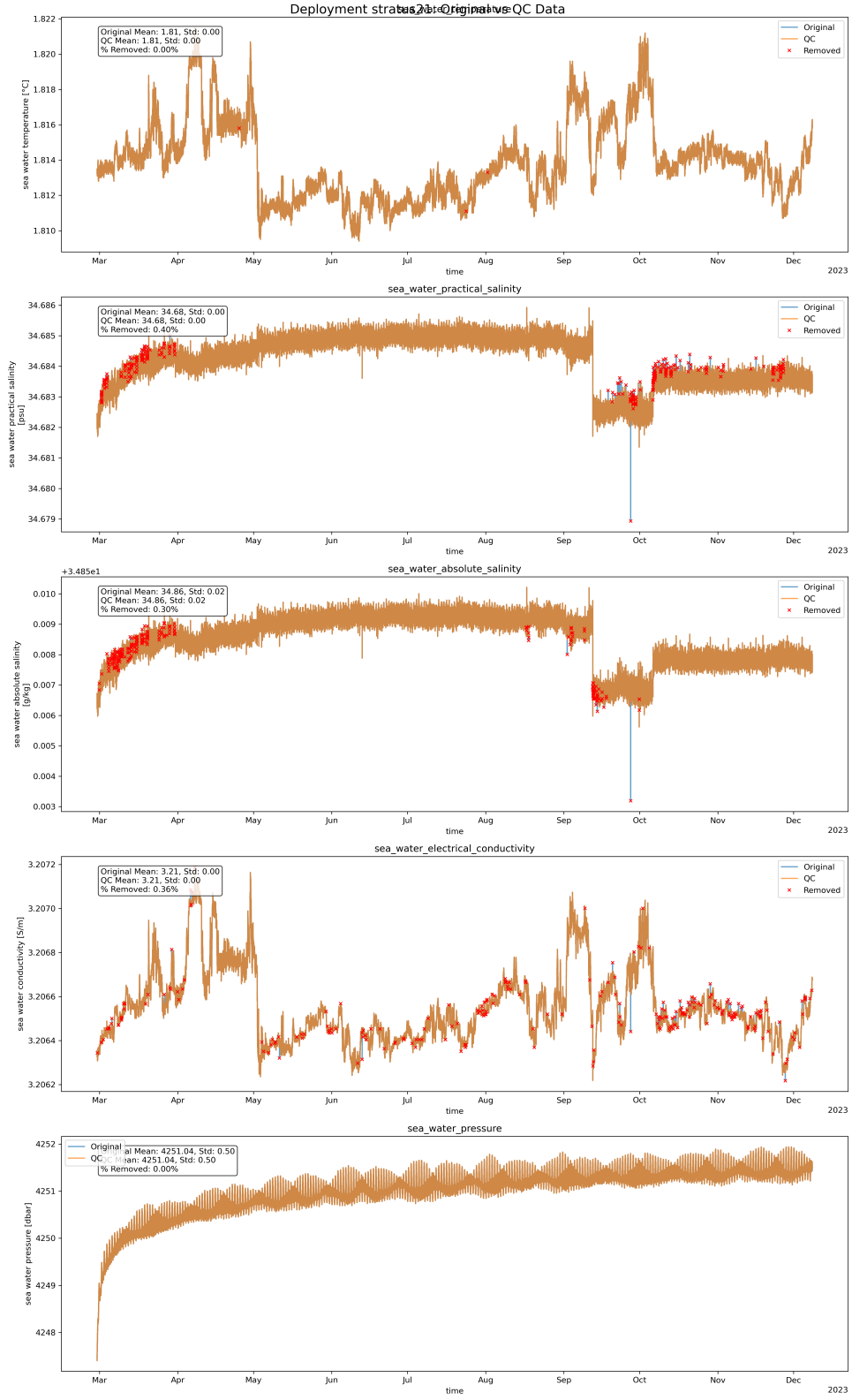
Figure 7: Original and clean plots of temperature, salinity, absolute salinity, conductivity, and pressure for instrument SBE37 11394 of stratus 21.
