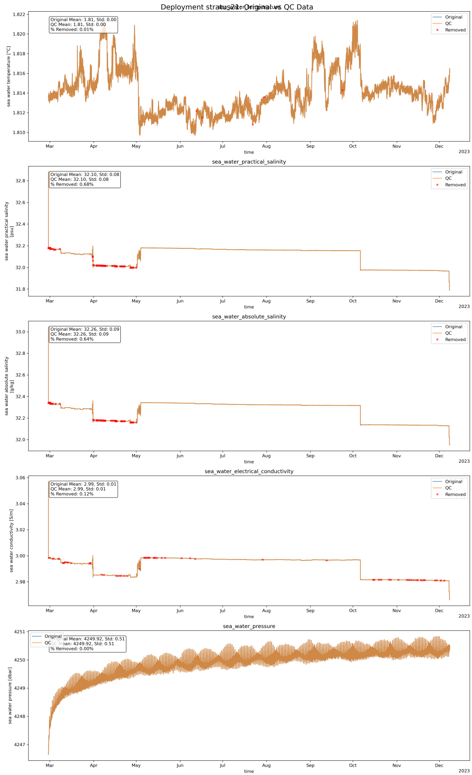
Figure 6: Original and clean plots of temperature, salinity, absolute salinity, conductivity, and pressure for instrument SBE37 11379 of stratus 21.
