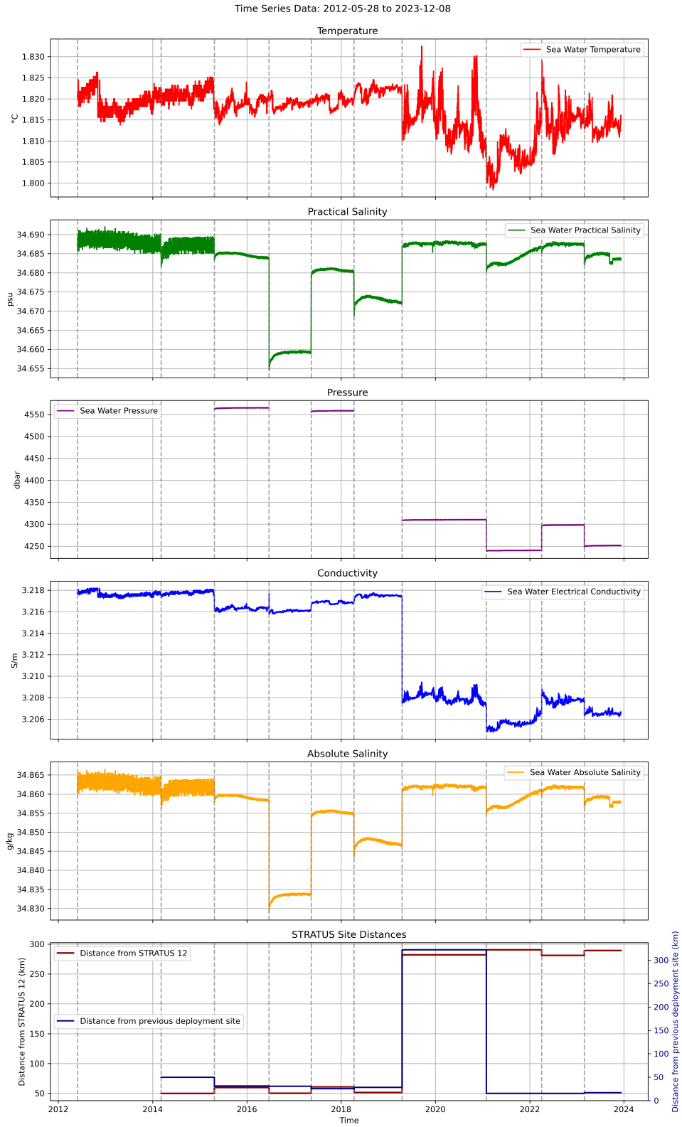
Figure 10: Merged dataset of stratus 12 to stratus 21 showing the transition at the merge point. This dataset combines data from the selected instrument (SBE37 10600) from stratus 20 and SBE37 11394 from stratus 21. This dataset incorporates all previous merges in the time series. The gray dashed line indicates the merge point between the two datasets.
