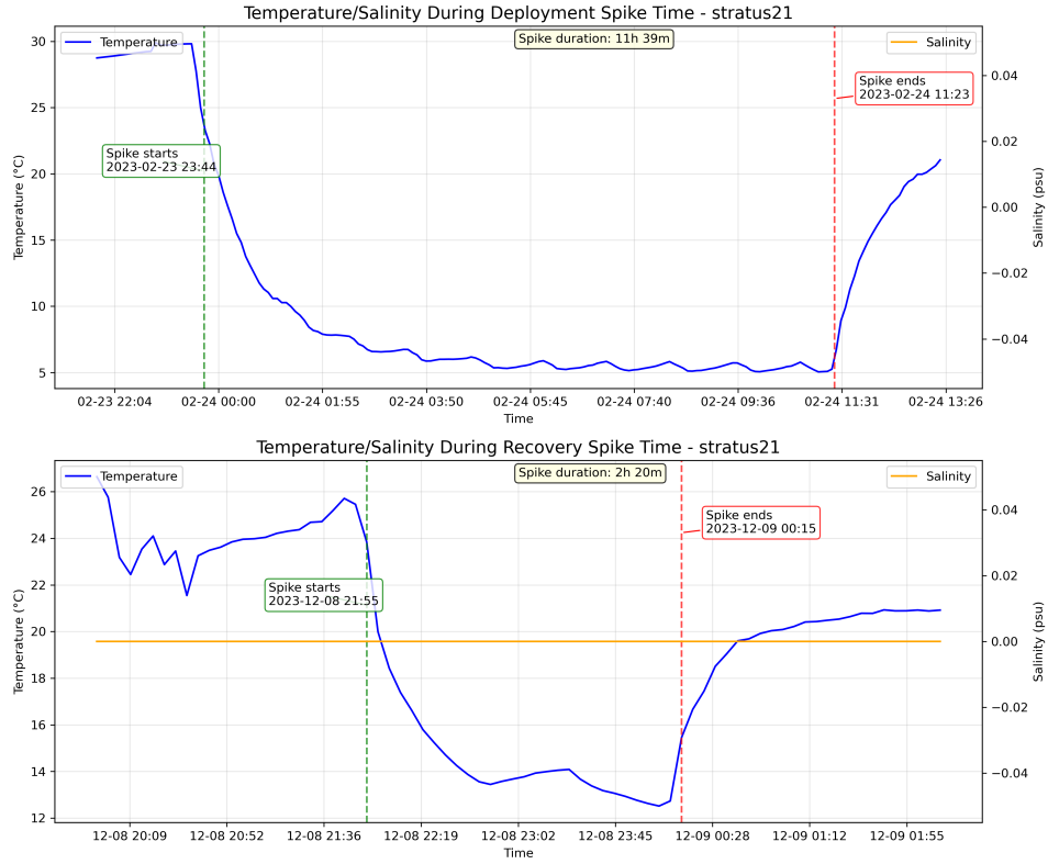
Figure 2: Deployment and recovery spike times for instrument SBE37 11394 of stratus 21 showing temperature changes during deployment and recovery operations. The vertical dashed lines indicate the recorded spike times (2023/02/24 11:23:00 for deployment and 2023/12/08 21:55:00 for recovery).
