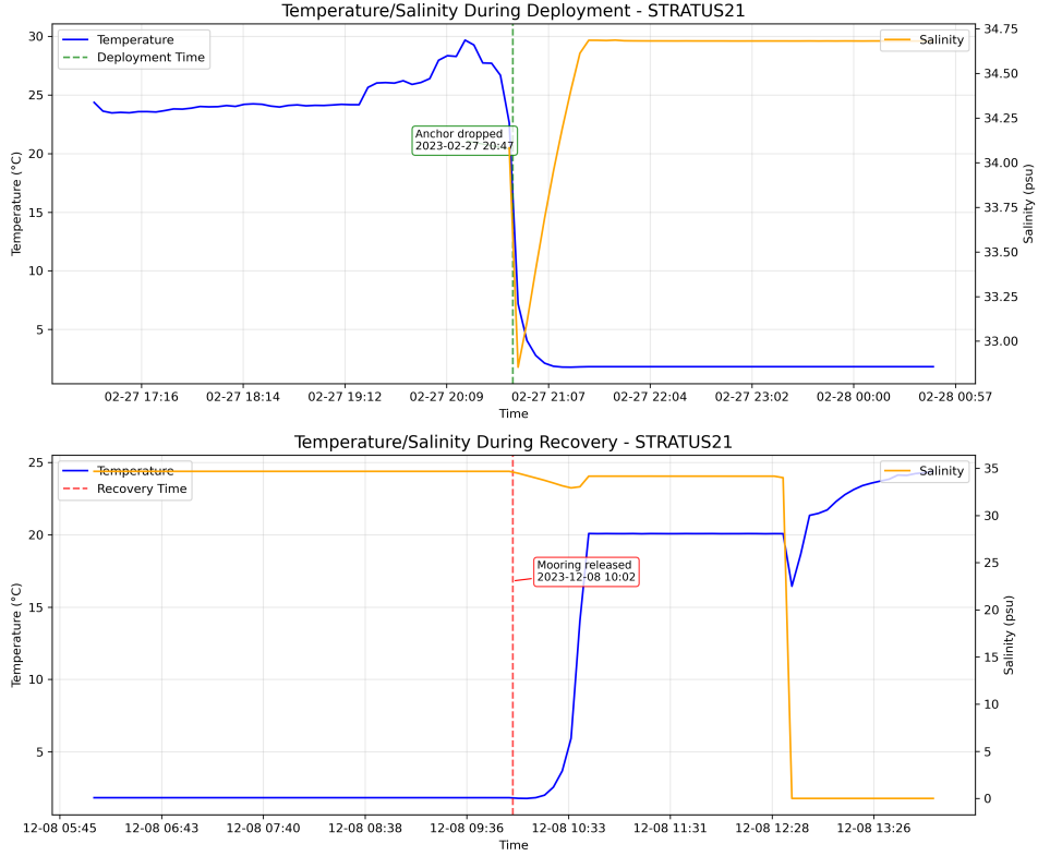
Figure 4: Detailed view of temperature changes during deployment and recovery phases for instrument SBE37 11394 of stratus 21.
