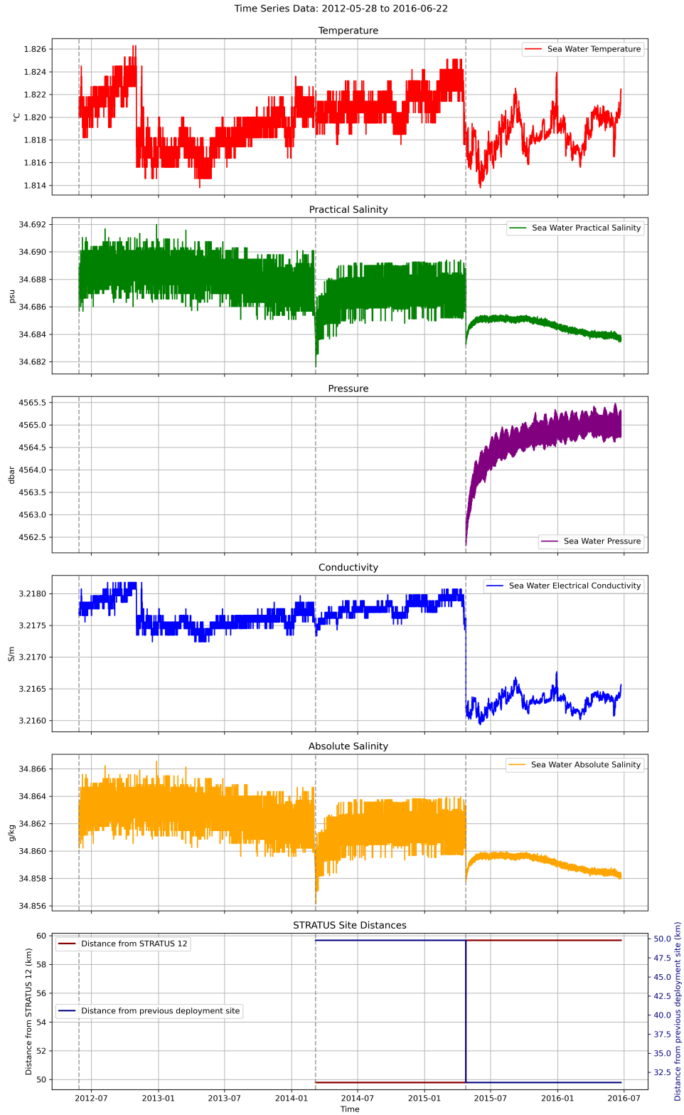
Figure 10: Merged dataset of stratus 12 to stratus 14 showing the seamless transition at the merge point. This dataset combines data from the selected instrument (SBE37 1875) from stratus 13 and SBE37 10600 from stratus 14. This dataset incorporates all previous merges in the time series. The gray dashed lines indicate the merge points.
