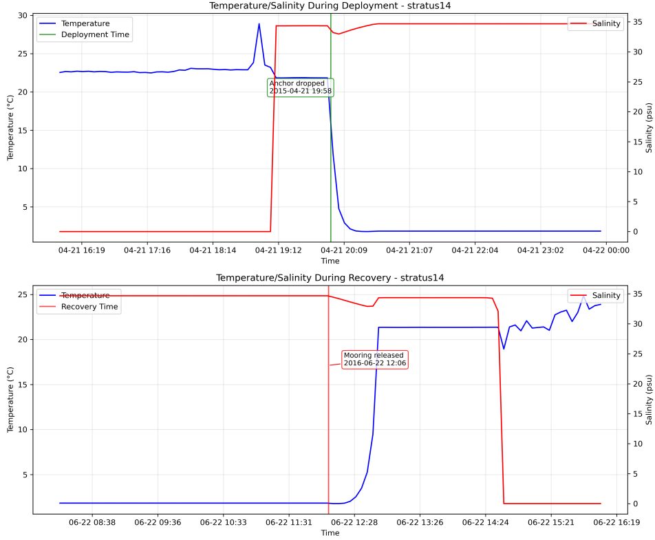
Figure 4: Detailed view of temperature changes during deployment and recovery phases for instrument SBE37 10601 of stratus 14.
