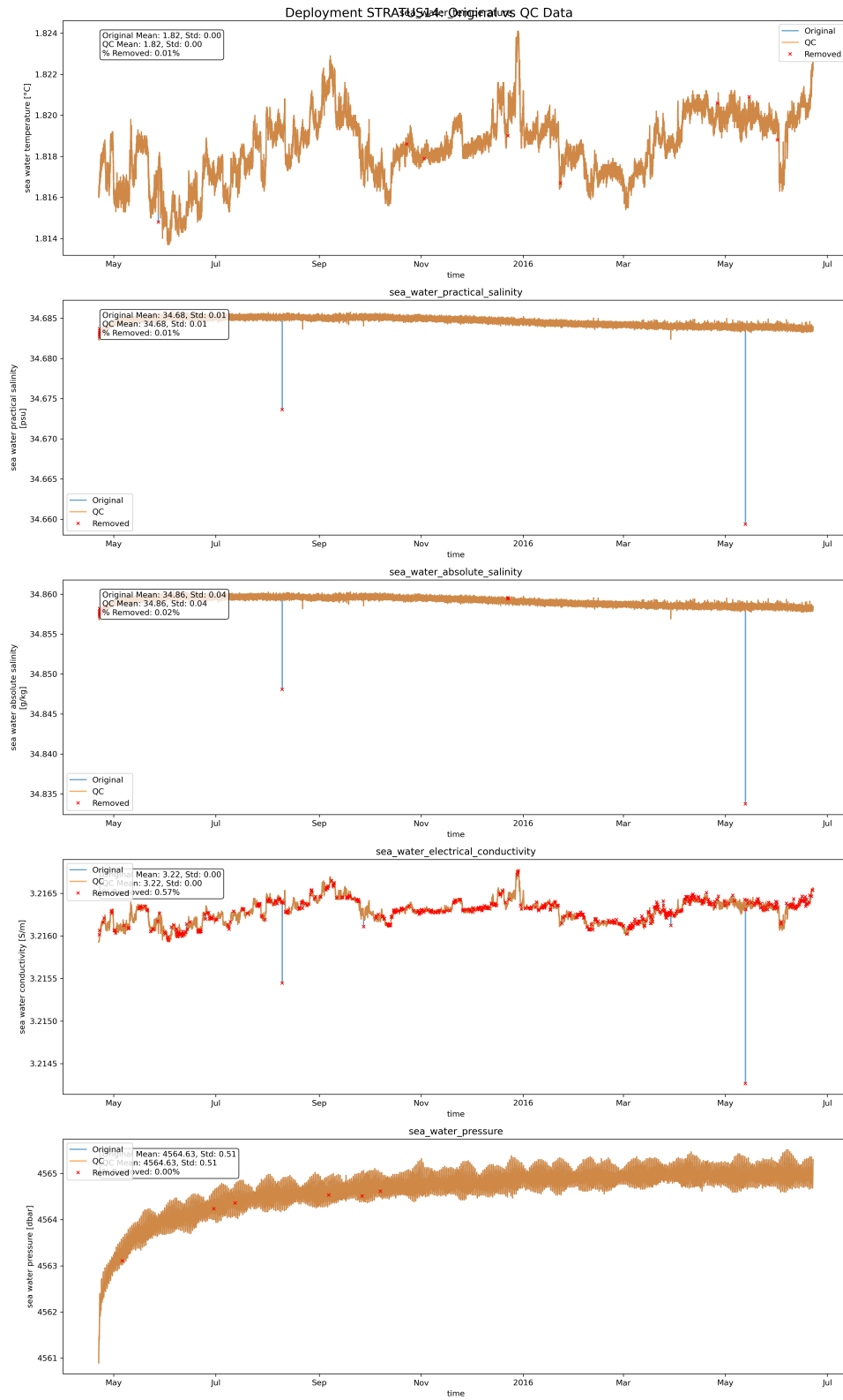
Figure 6: Original and clean plots of temperature, salinity, absolute salinity, conductivity, and pressure for instrument SBE37 10600 of stratus 14.
