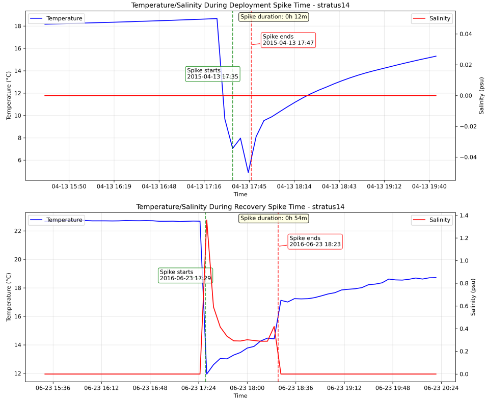
Figure 2: Deployment and recovery spike times for instrument SBE37 10601 of stratus 14 showing temperature changes during deployment and recovery operations. The vertical dashed lines indicate the recorded spike times (04/13/2015 17:35 for deployment and 06/23/2016 17:29 for recovery).
