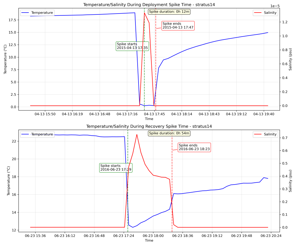
Figure 1: Deployment and recovery spike times for instrument SBE37 10600 of stratus 14 showing temperature changes during deployment and recovery operations. The vertical dashed lines indicate the recorded spike times (04/13/2015 17:35 for deployment and 06/23/2016 17:29 for recovery).
