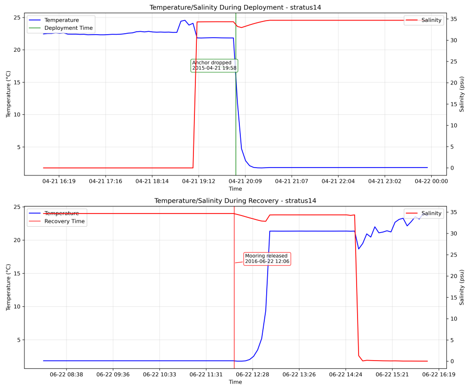
Figure 3: Detailed view of temperature changes during deployment and recovery phases for stratus 14, showing instrument SBE37 10600.
