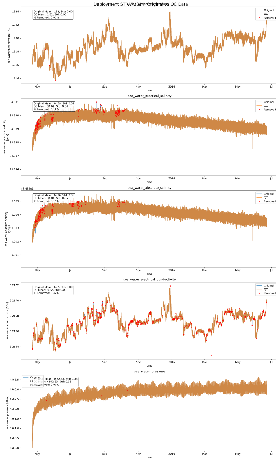
Figure 7: Original and clean plots of temperature, salinity, absolute salinity, conductivity, and pressure for instrument SBE37 10601 of stratus 14.
